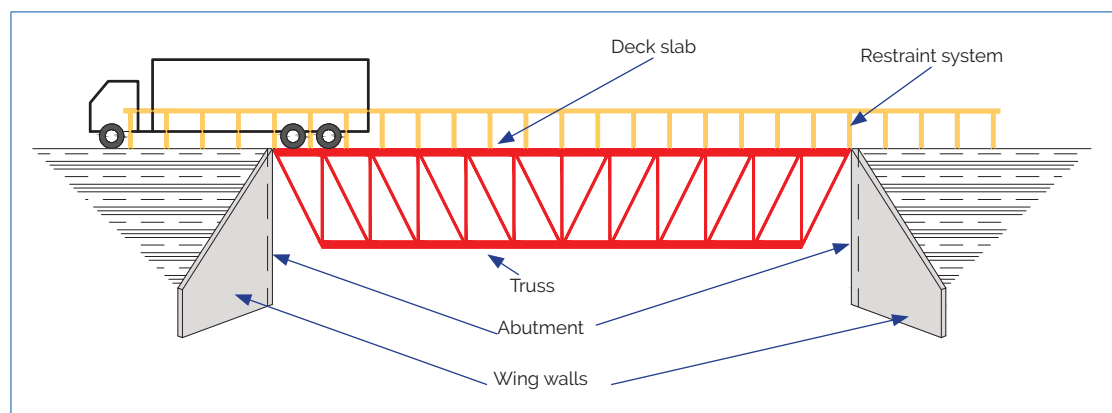
Figure 4.3 Cross-section of an underslung truss bridge
