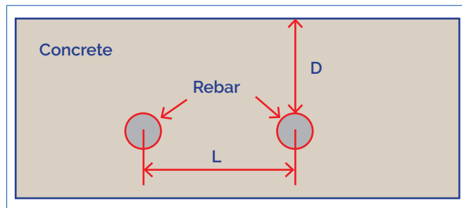
Figure 7.15 Measuring conditions related concrete depth and spacing
