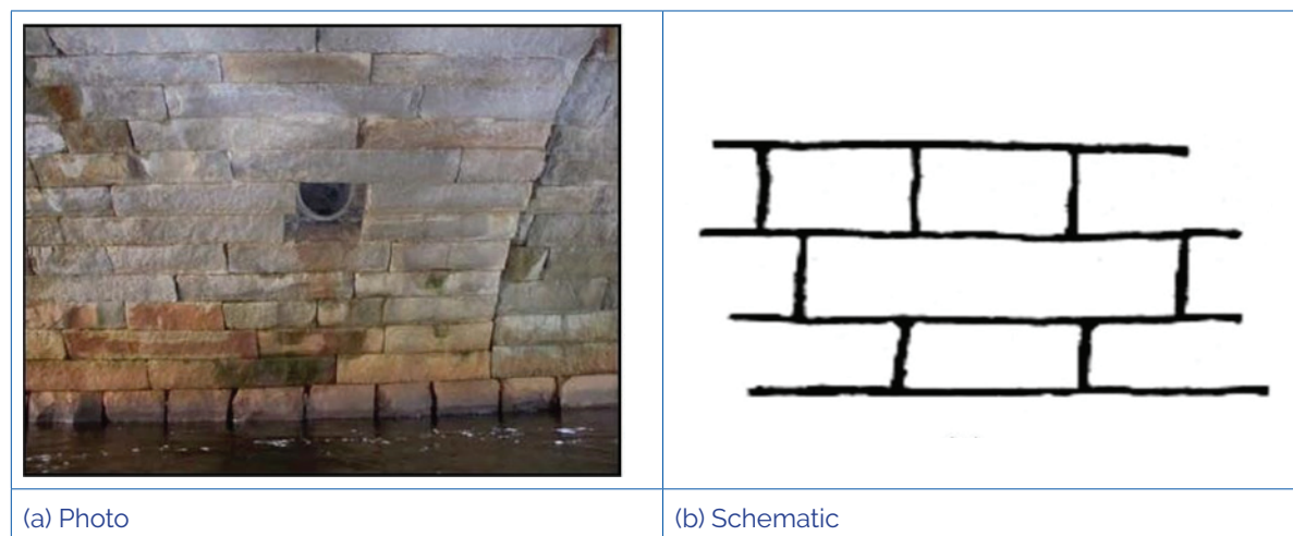
Figure 2.27 Coursed ashlar masonry
