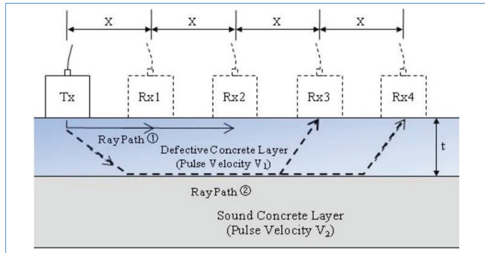
Figure 7.10 Sampling pattern for investigation of scaling, delamination
