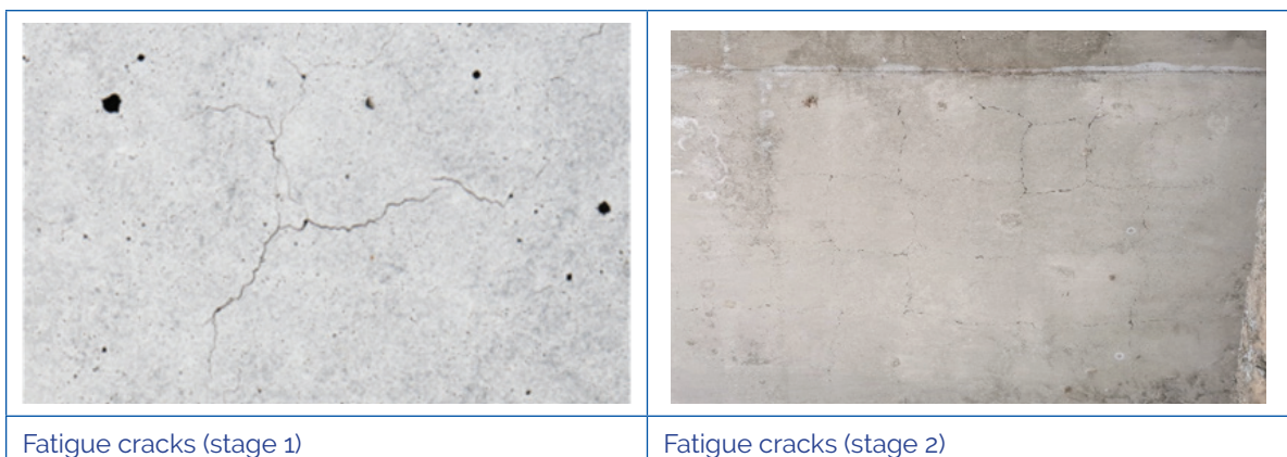
Figure 3.20 Progression of fatigue
