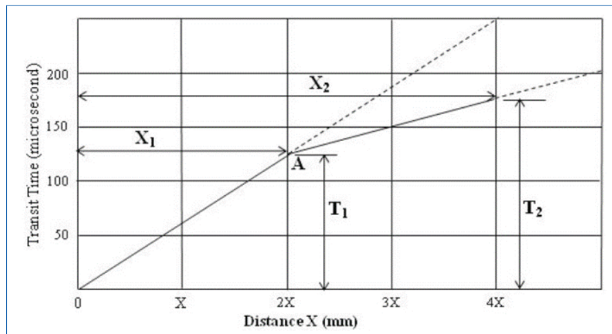
Figure 7.11 Plot of transit time versus distance
