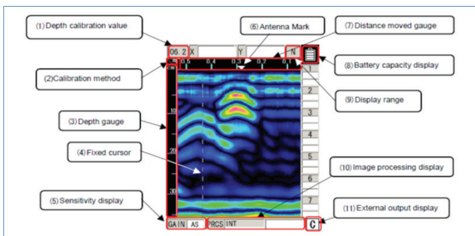
Figure 7.18 Example of a test scan
