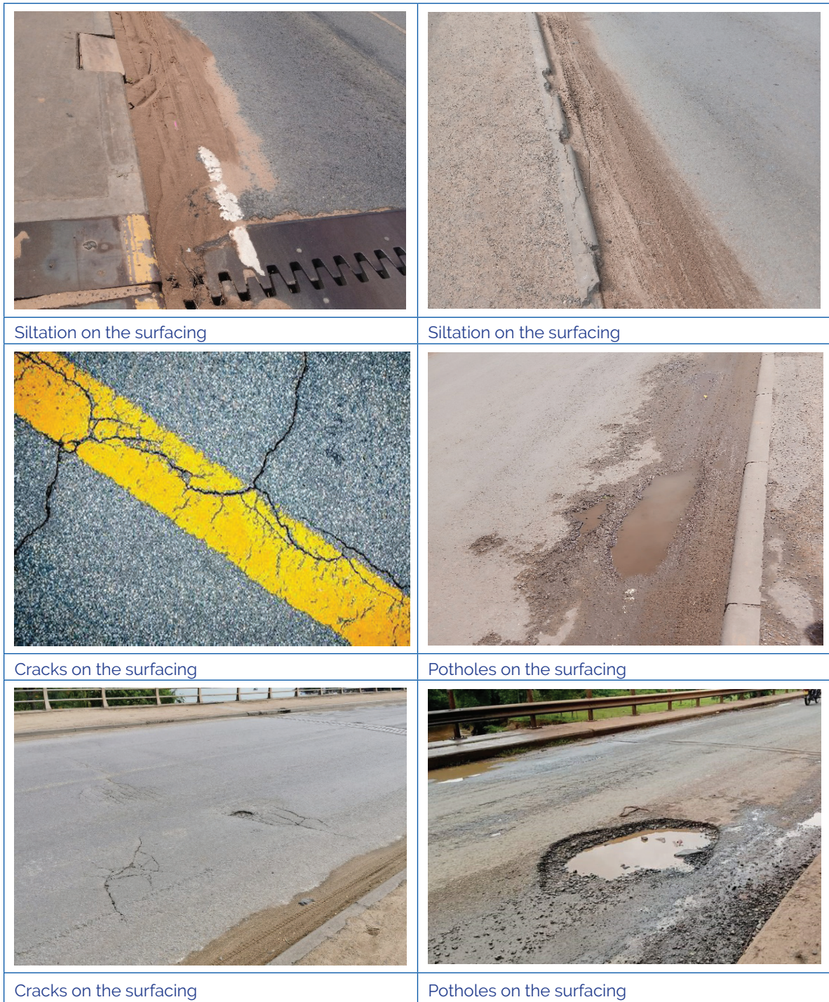
Figure 3.64 Sample photos of surface deteriorations
