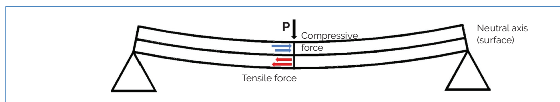
Figure 2.11 Behaviour of a member due to bending forces
