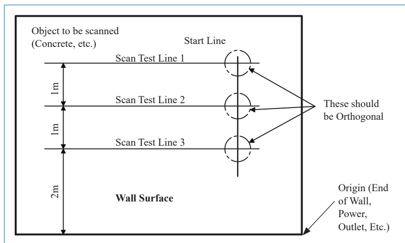
Figure 7.16 Example of scan test set-up
