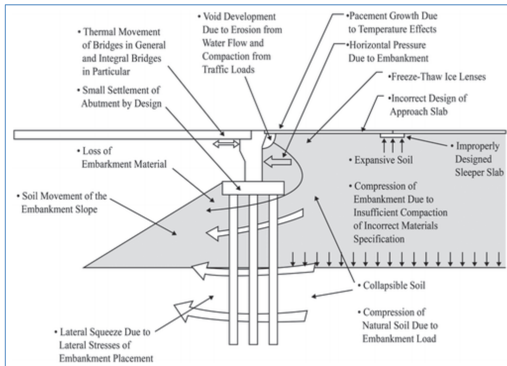
Figure 3.78 Sample diagram showing the causes of settlement of an approach slab
