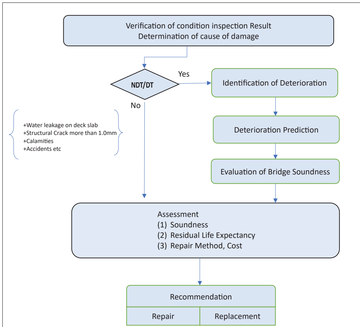
Figure 4.4 Flow chart of assessment for bridge engineering inspection
