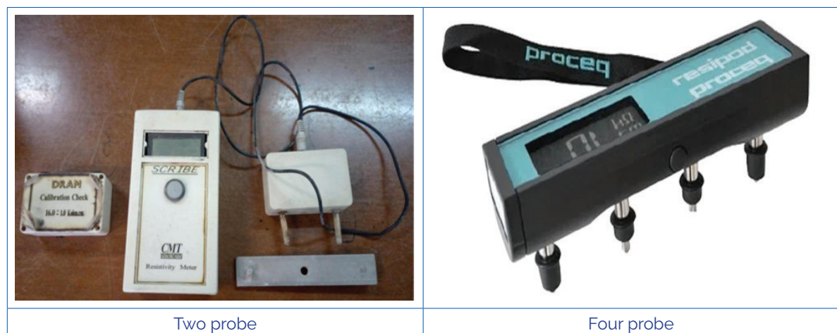
Figure 7.29 Two and four probe resistivity meter
