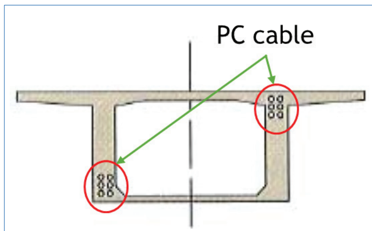
Figure 2.17 PC inner cable location
