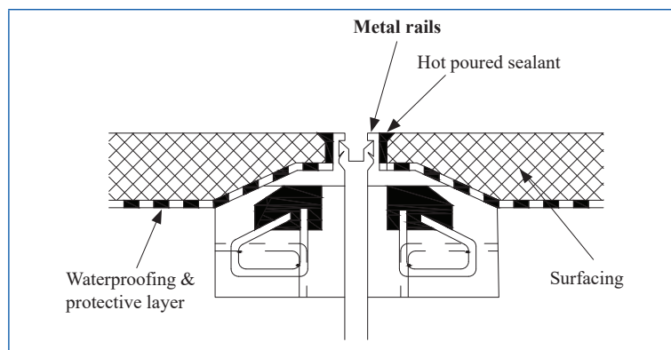
Figure 3.71 Cast-in (single element)
