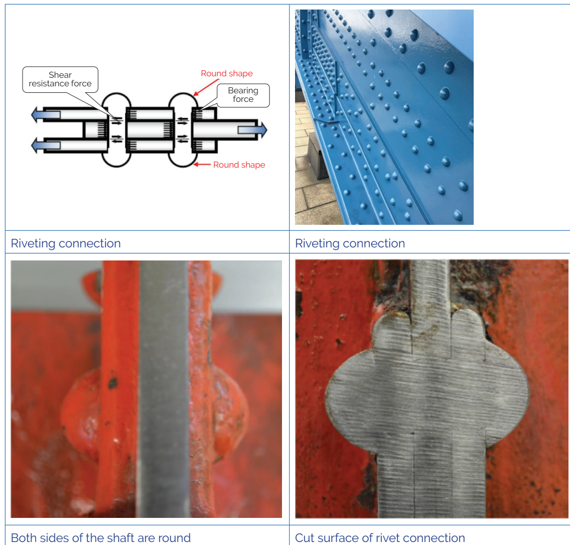
Figure 2.25 Riveting connection
