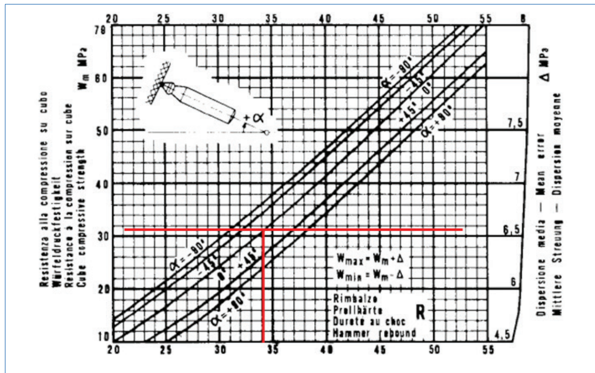
Figure 7.4 Rebound value and cube compressive strength chart
