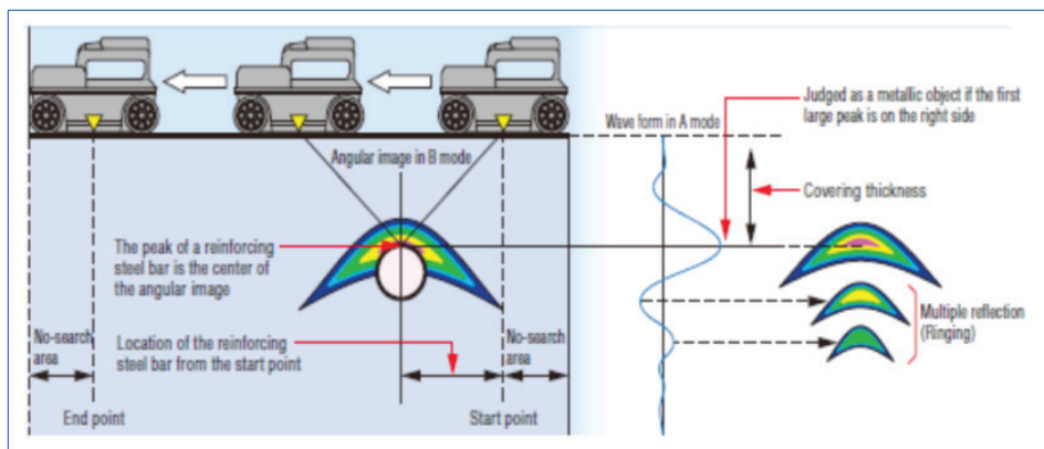
Figure 7.17 Scanning diagram
