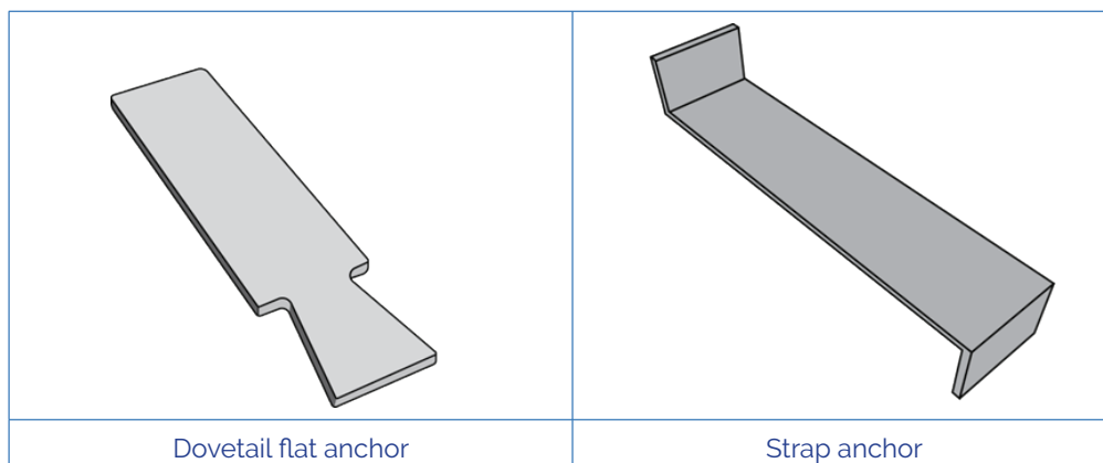
Figure 2.36 Masonry anchor types
