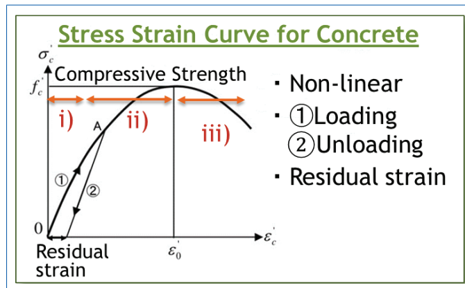
Figure 2.13 Stress-strain curve for concrete
