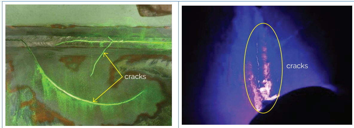
Figure 7.47 Detection of crack by magnetic particle testing
