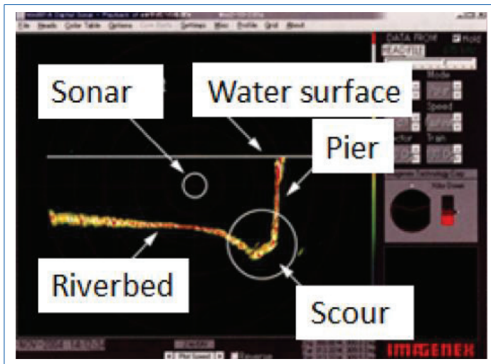
Figure 7.38 Screen image of SONAR test
