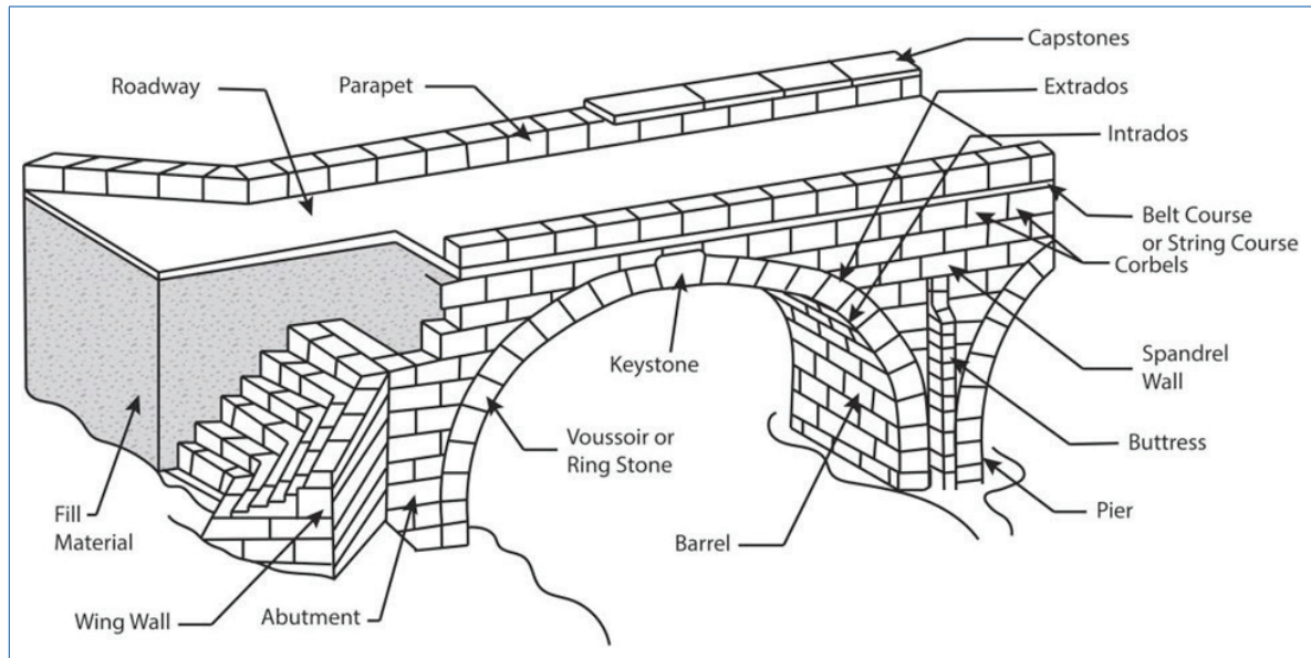
Figure 2.30 Arch elements
