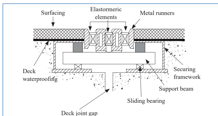
Figure 3.72 Cast-in (multiple element)
