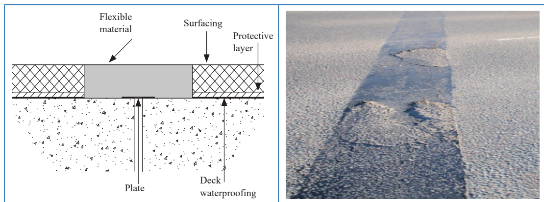
Figure 3.67 Asphaltic plug joint
