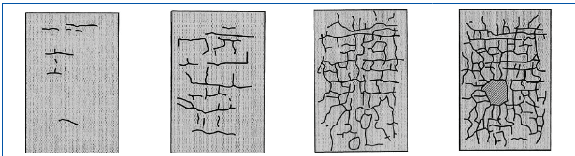
Figure 3.20 Progression of fatigue
