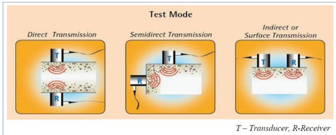
Figure 7.6 Placing of the two transducers
