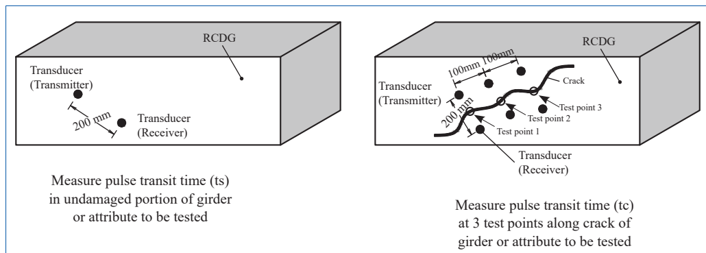
Figure 7.9 Measuring pulse transit time
