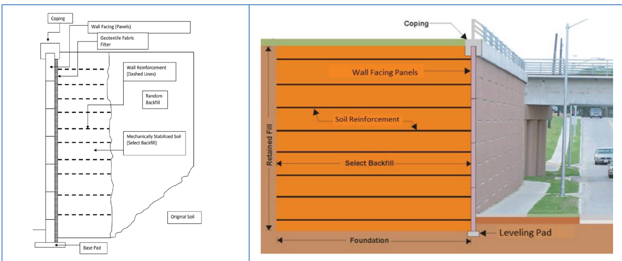
Cross section of reinforced earth retaining wall
