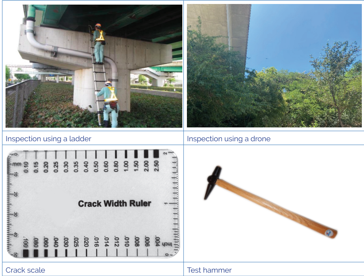
Figure 5.3 Tools and equipment for inspection
