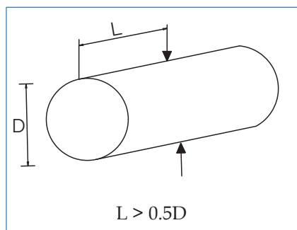
Figure 7.58 Core configuration for diametrical test
