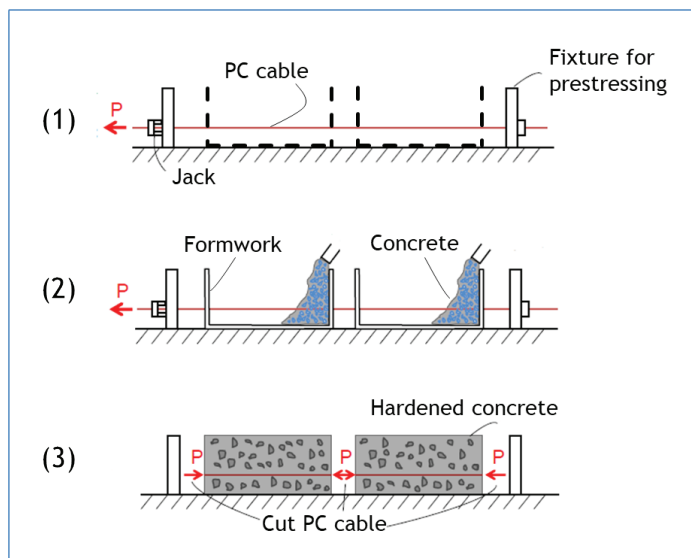
Figure 2.15 Pre-tensioning process
