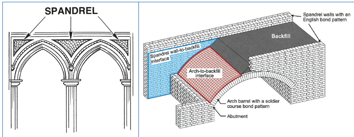
Figure 3.56 Cross section of arch bridge
