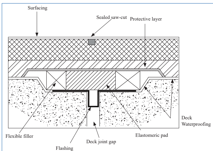
Figure 3.66 Buried joint
