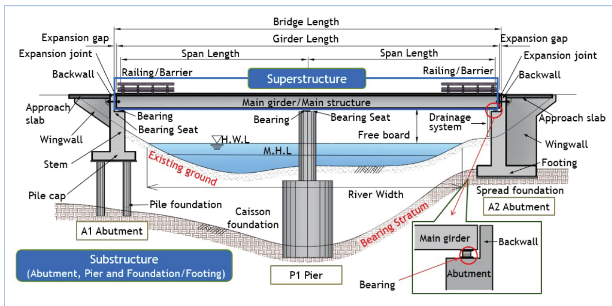
Figure 2.1 Bridge components
