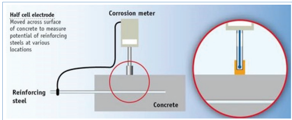
Figure 7.34 Testing diagram
