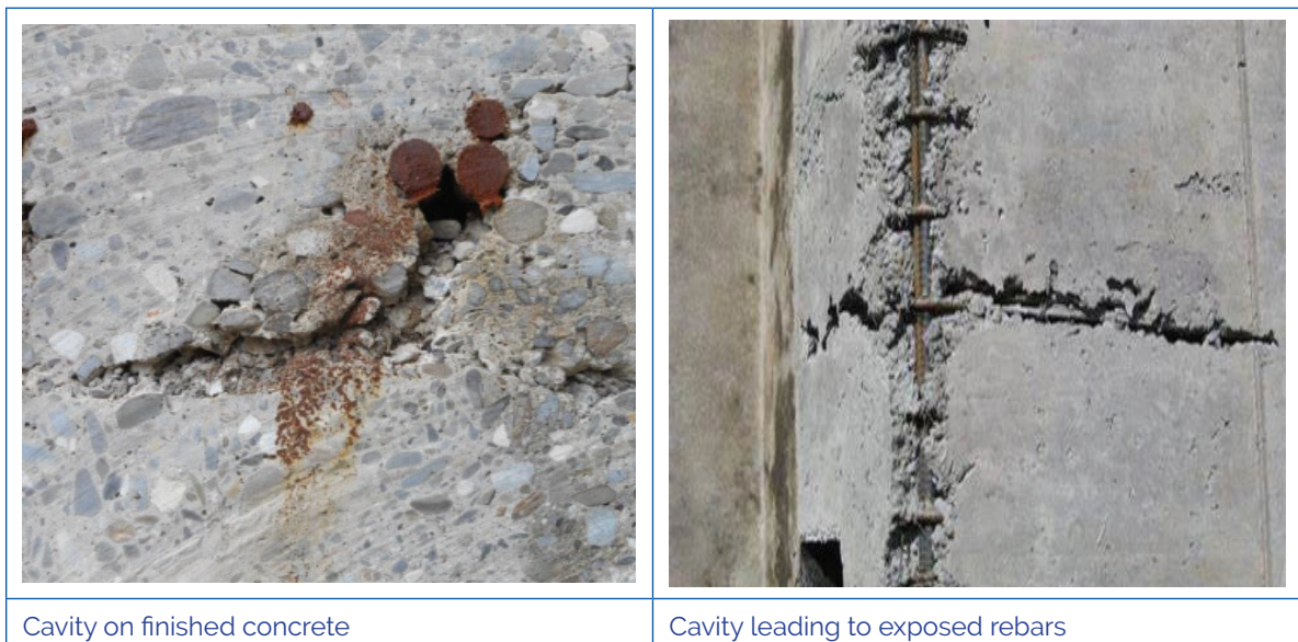
Figure 3.27 Sample photos of cavity
