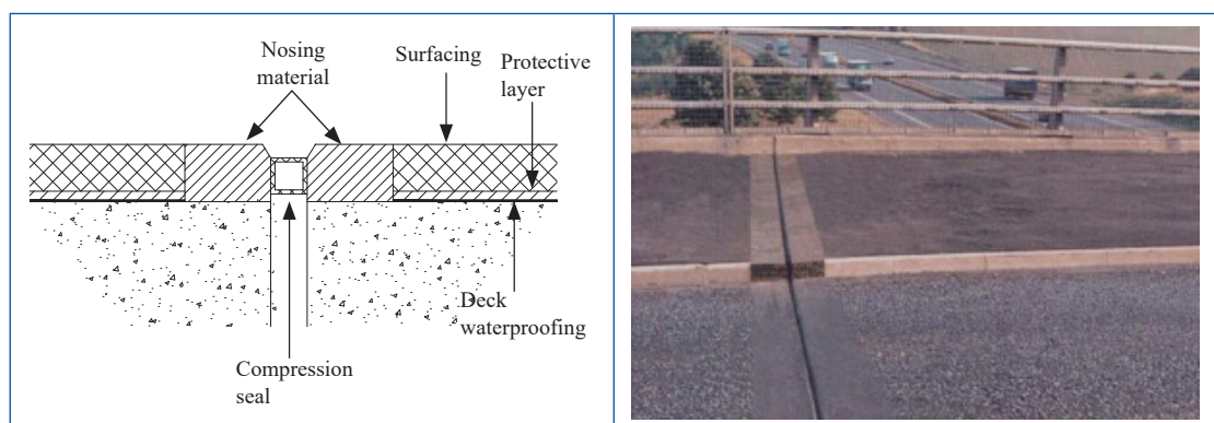
Figure 3.68 Nosing joint
