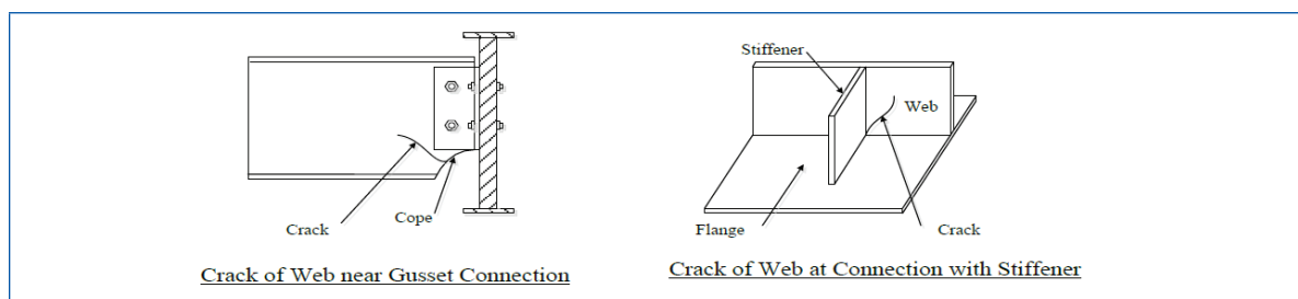
Figure 3.34 Common crack locations in steel members
