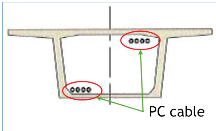
Figure 2.18 PC outer cable location
