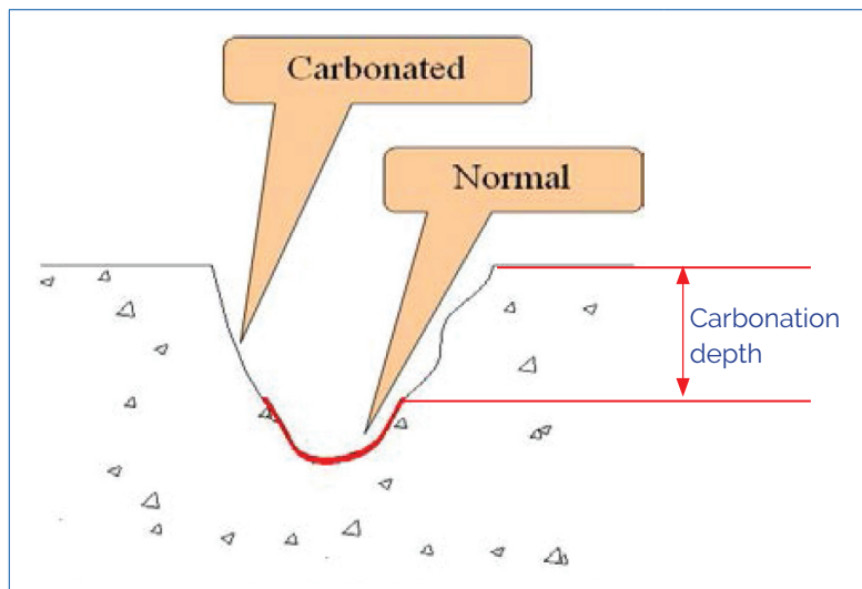
Figure 7.53 Measurement of carbonation depth on chipped off concrete surface
