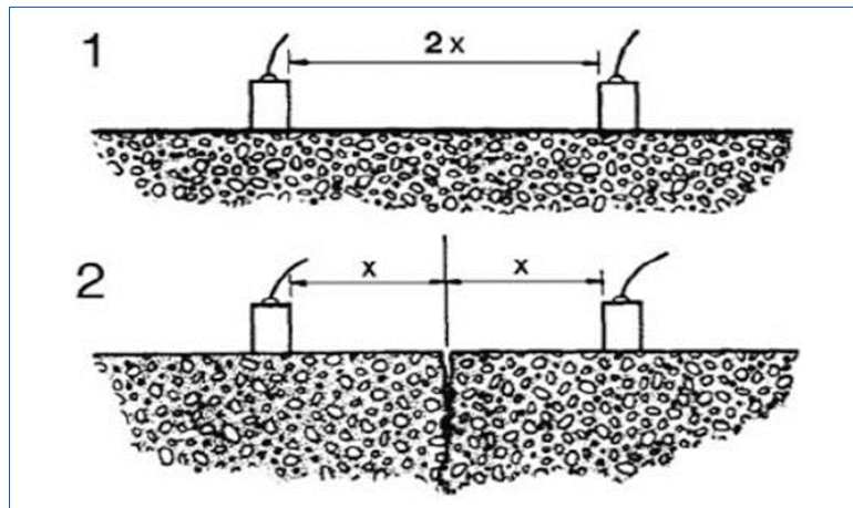
Figure 7.8 Transducers positioning for estimation of crack depth
