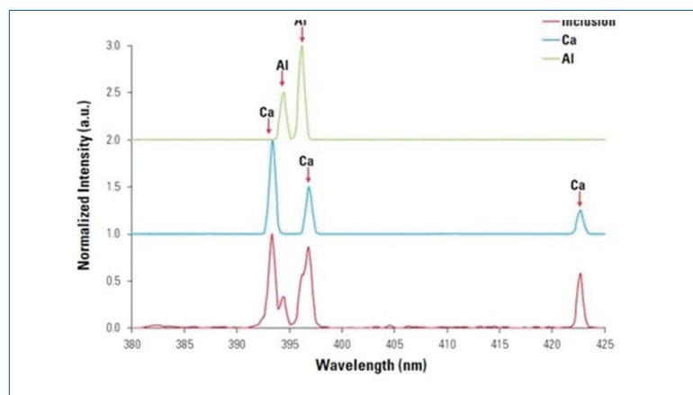
Figure 7.66 A spectrograph showing the intensity of chemicals present in a steel sample
