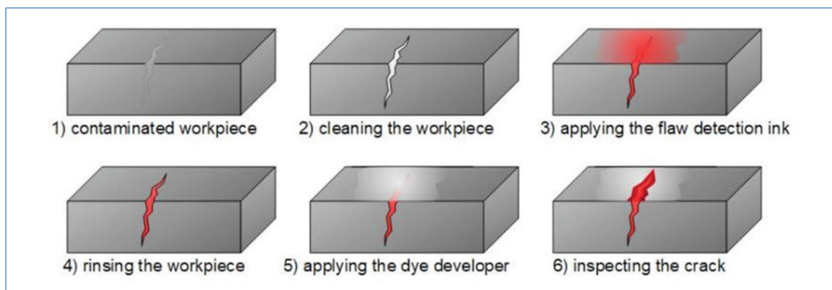
Figure 7.50 Indications of the surface discontinuities or flaws
