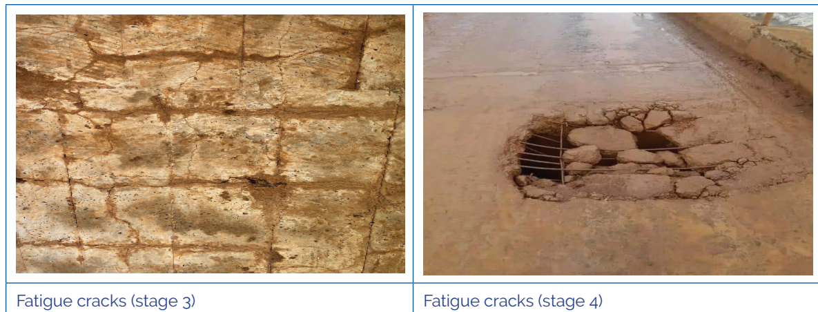
Figure 3.21 Sample photos of fatigue
