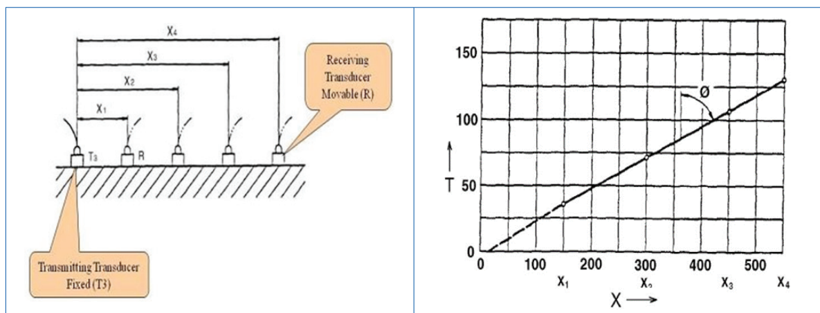
Figure 7.7 Indirect (surface) transmission
