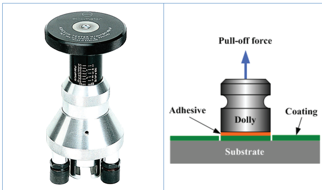
Figure 7.64 Equipment for pull-off test
