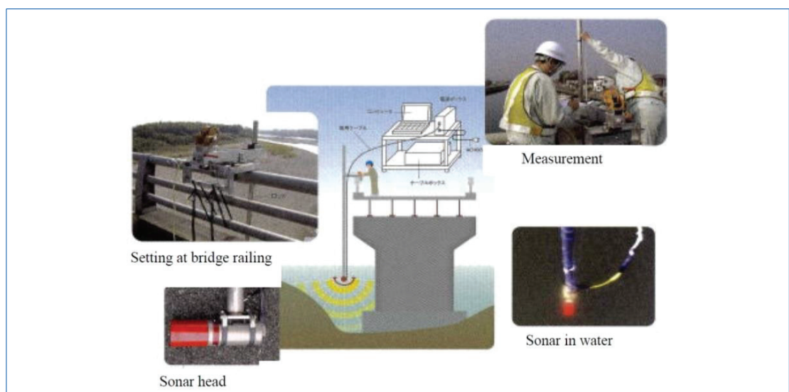
Figure 7.37 System configuration
