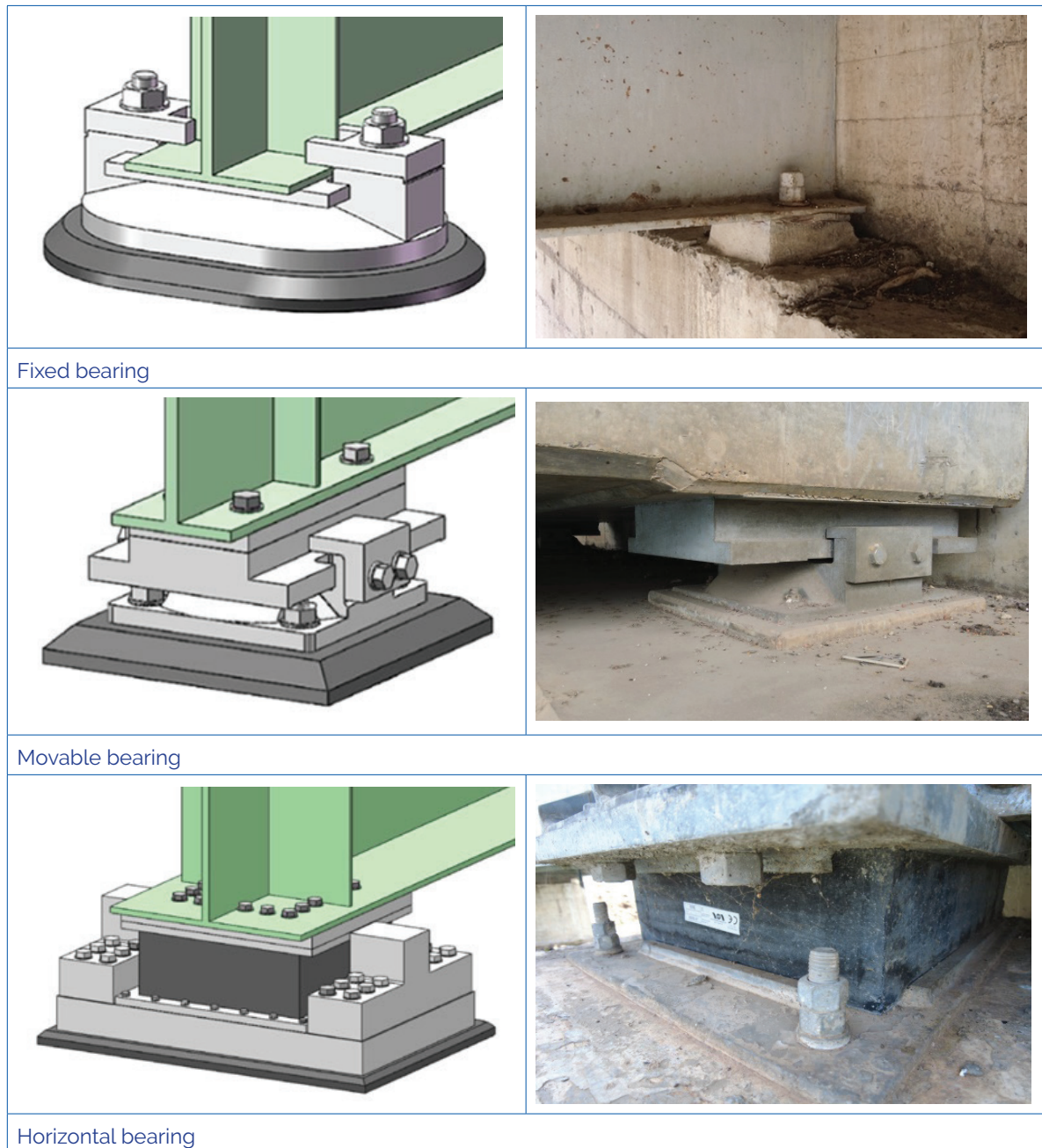
Figure 2.26 Types of bearings
