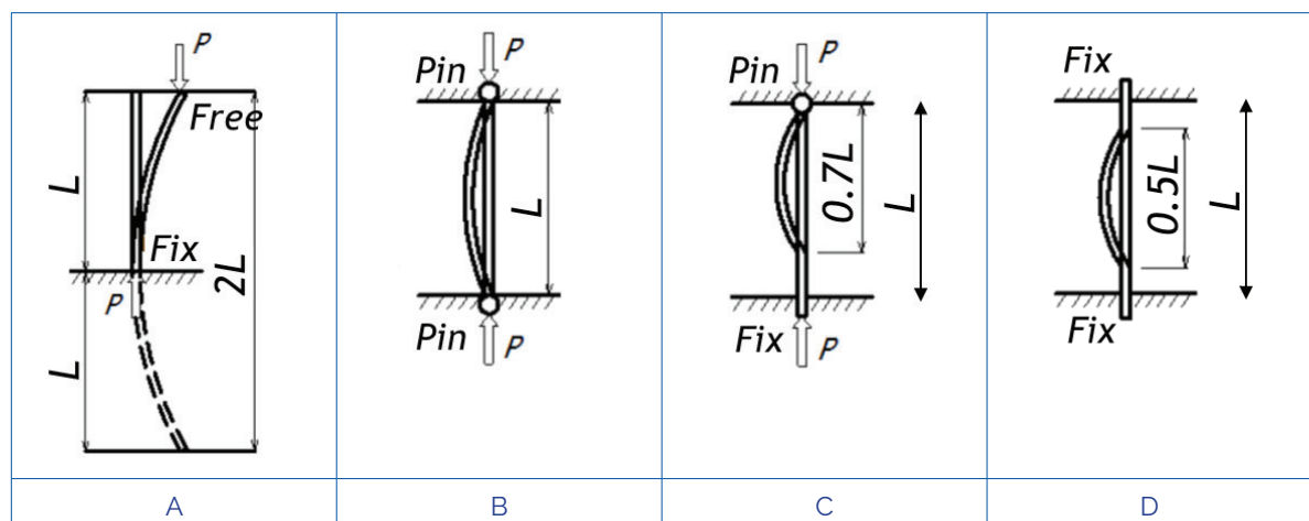
Figure 2.20 Design to prevent buckling
