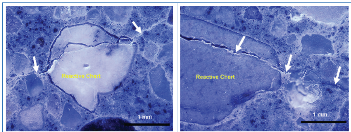
Figure 7.61 Cracks from reactive chert fine aggregate particles into paste
