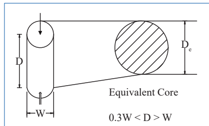
Figure 7.59 Core configuration for axial test
