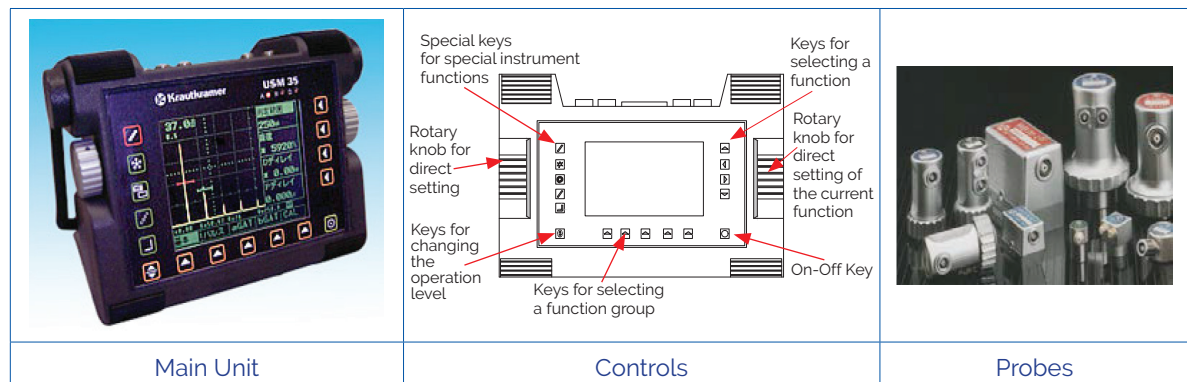
Figure 7.42 Ultrasonic flaw detector
