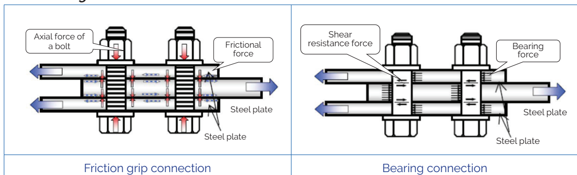
Figure 2.24 High tension bolt connection
