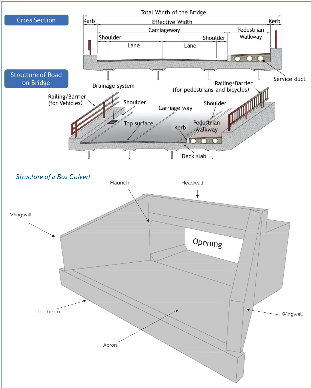
Figure 2.2 Structure of road on bridges and box culvert
