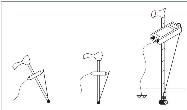
Figure 7.33 Set-up for surveys on horizontal surfaces such as bridge decks/slabs etc.
