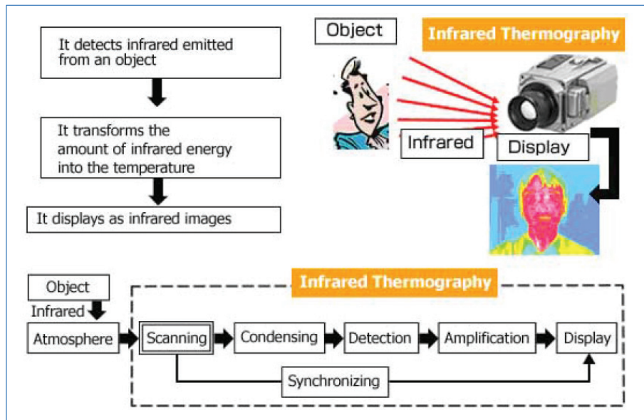
Figure 7.21 Process of thermal imaging
