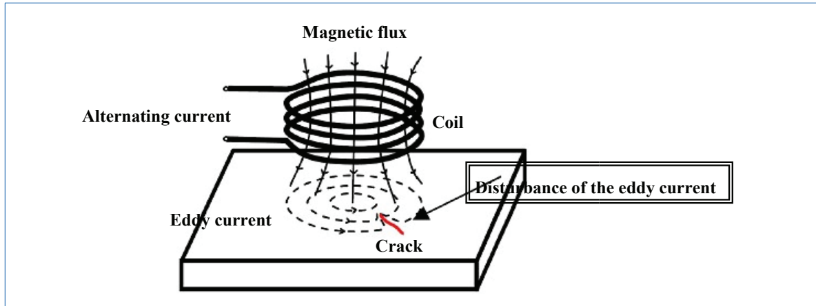
Figure 7.48 Eddy current testing
