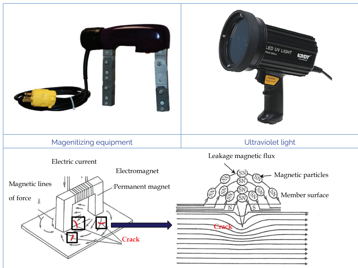
Figure 7.46 Magnetic particle testing
