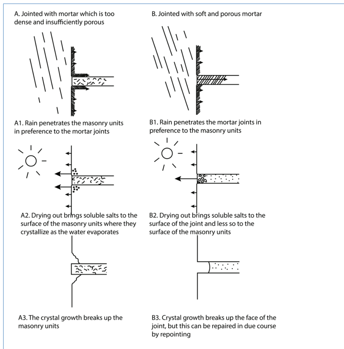
Figure 2.34 Benefits of hard and soft mortar
