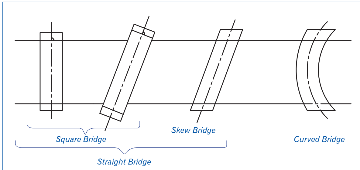
Figure 2.7 Classification by bridge plan shape
