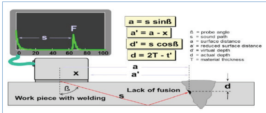
Figure 7.44 Testing of flaws
