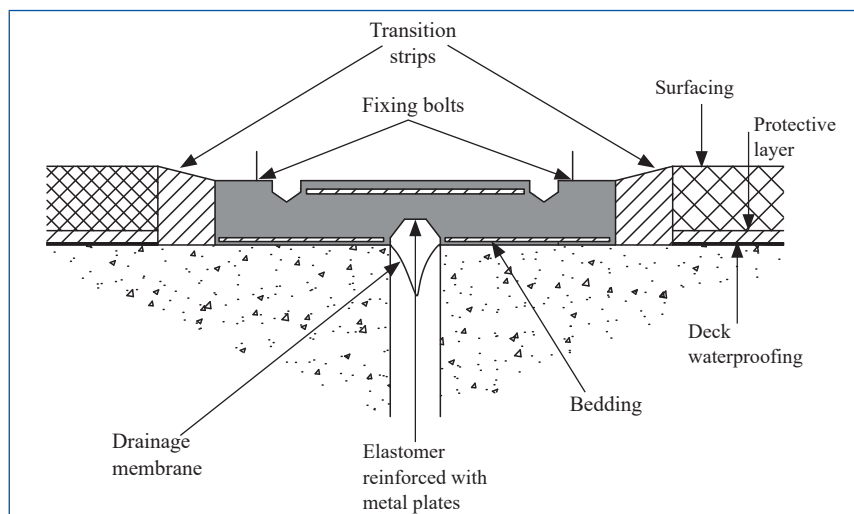
Figure 3.69 Reinforced elastomeric joint
