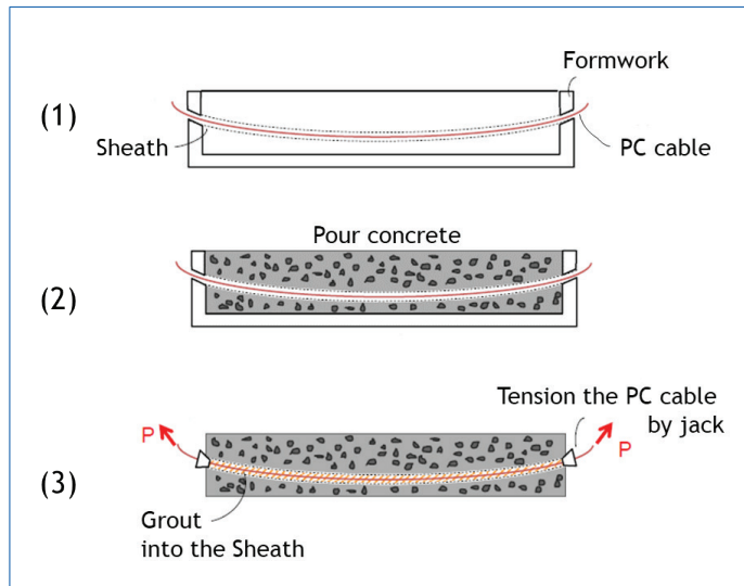
Figure 2.16 Post-tensioning process
