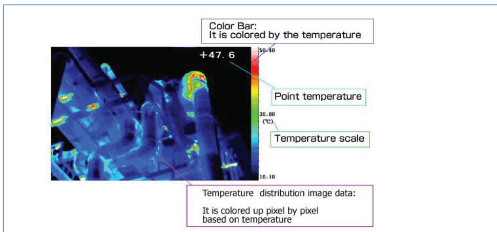
Figure 7.23 Sample image from infrared camera
