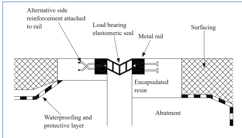
Figure 3.73 Resin encapsulated joint
