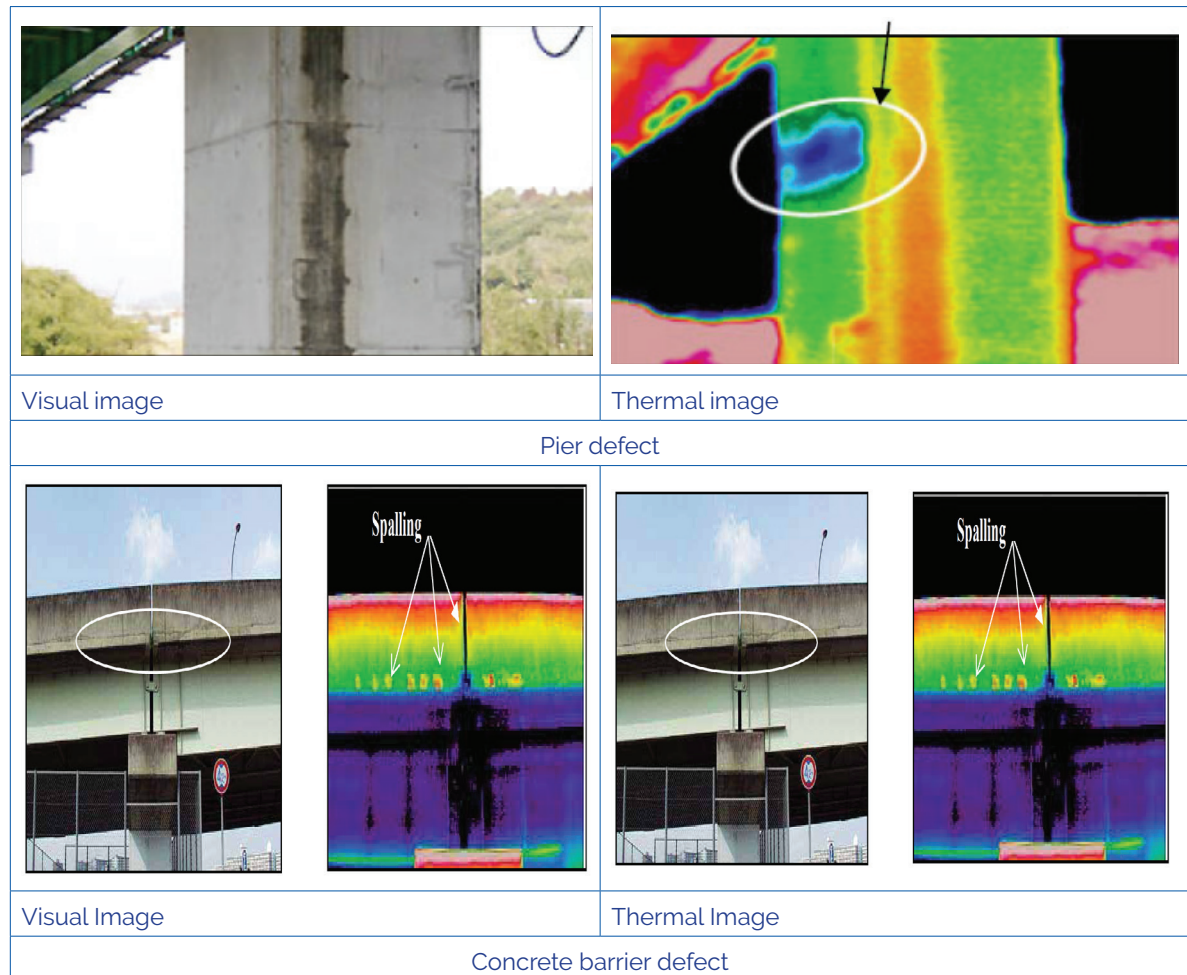
Figure 7.24 Examples of defects detection using infrared thermal imaging
