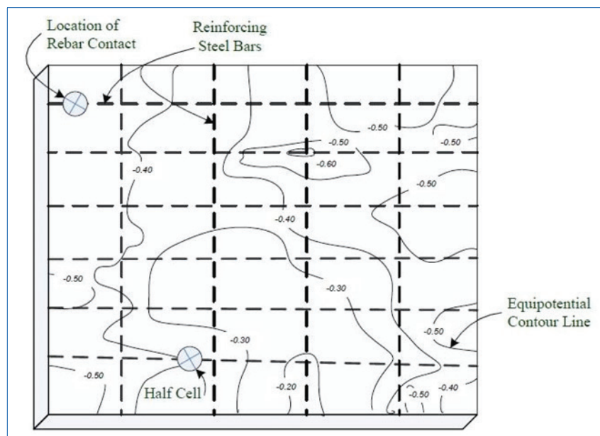
Figure 7.35 Example of equi-potential contour map
