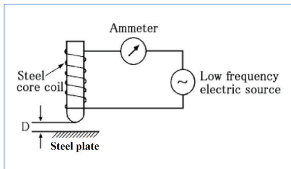
Figure 7.39 Principle of coating thickness measurement on surface of steel plate
