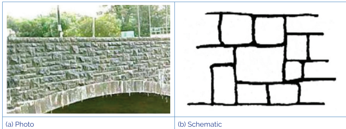
Figure 2.28 Random ashlar masonry
