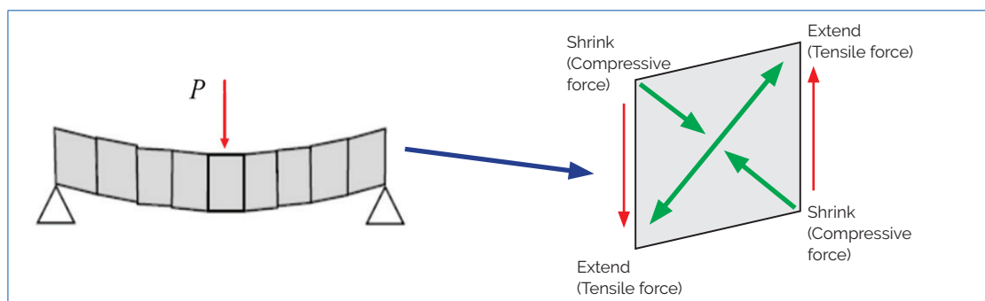
Figure 2.12 Member under shear force
