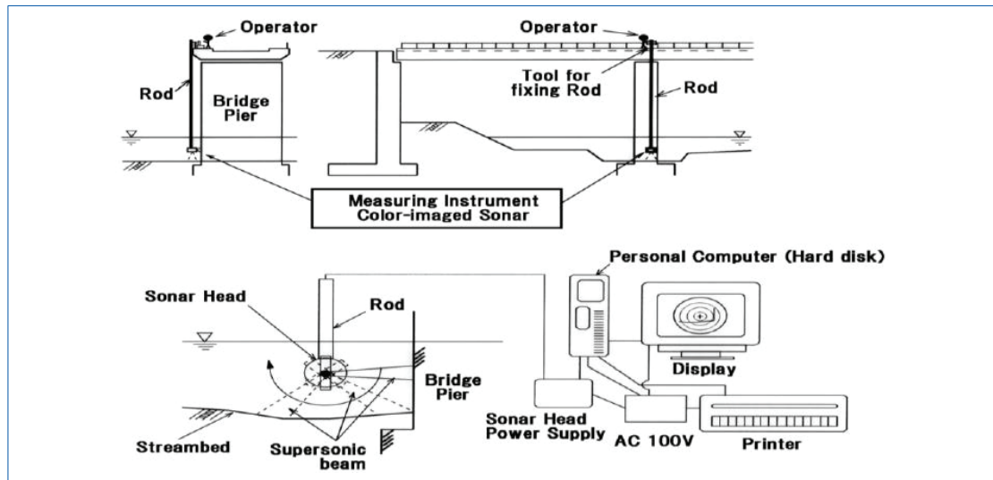
Figure 7.36 Outline of SONAR testing
