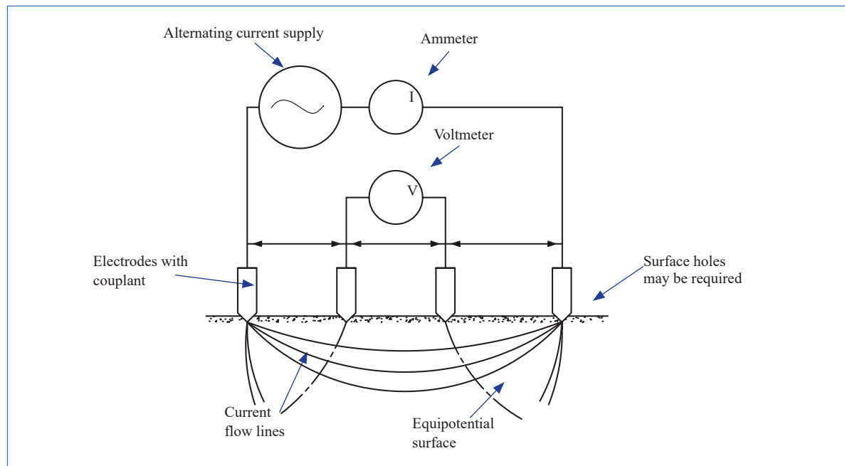
Figure 7.30 Schematic of Wenner 4 probe resistivity meter
