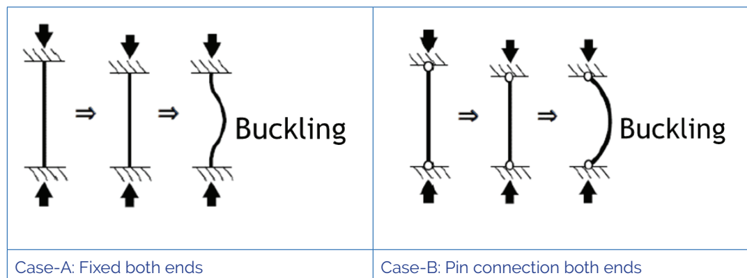
Figure 2.19 Buckling in steel
